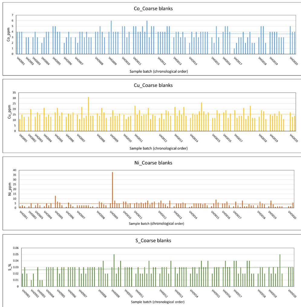
Figure 8-4 Coarse blank analysis results of the 2020 FinnCobalt drilling campaign, sorted by submitted sample batch in chronological order.
