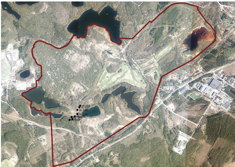
Figure 7-3 Overview map of the 2017-2018 FinnCobalt (Vulcan Resources) drilling in relation to the mining concession.
