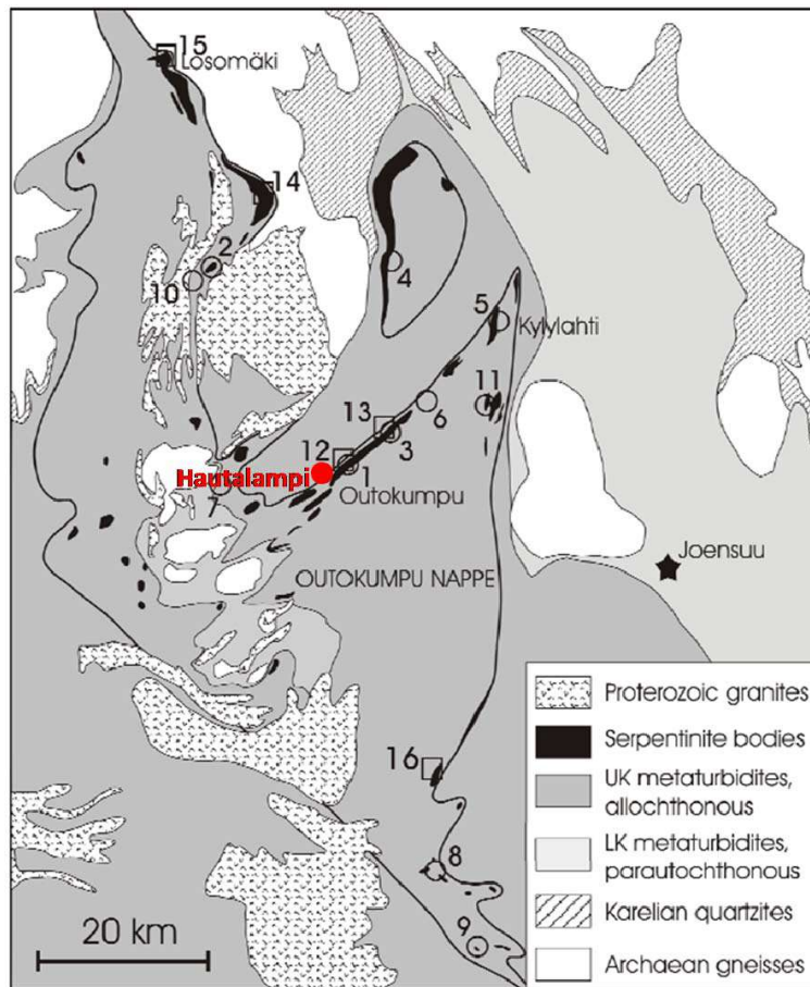
Figure 6-1 Map of the Outokumpu type sulphide deposits in North Karelia
