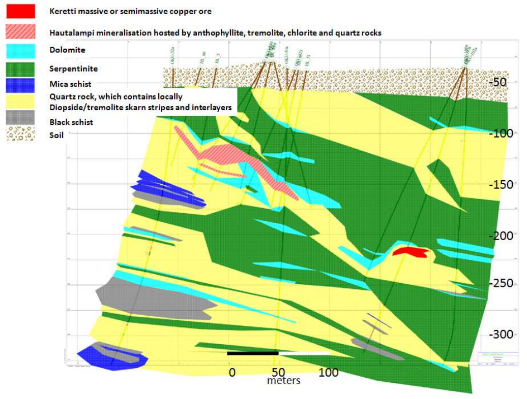
Figure 6-3 Cross-section through profile 92 of the Keretti copper (Outokumpu) and Hautalampi deposits.
