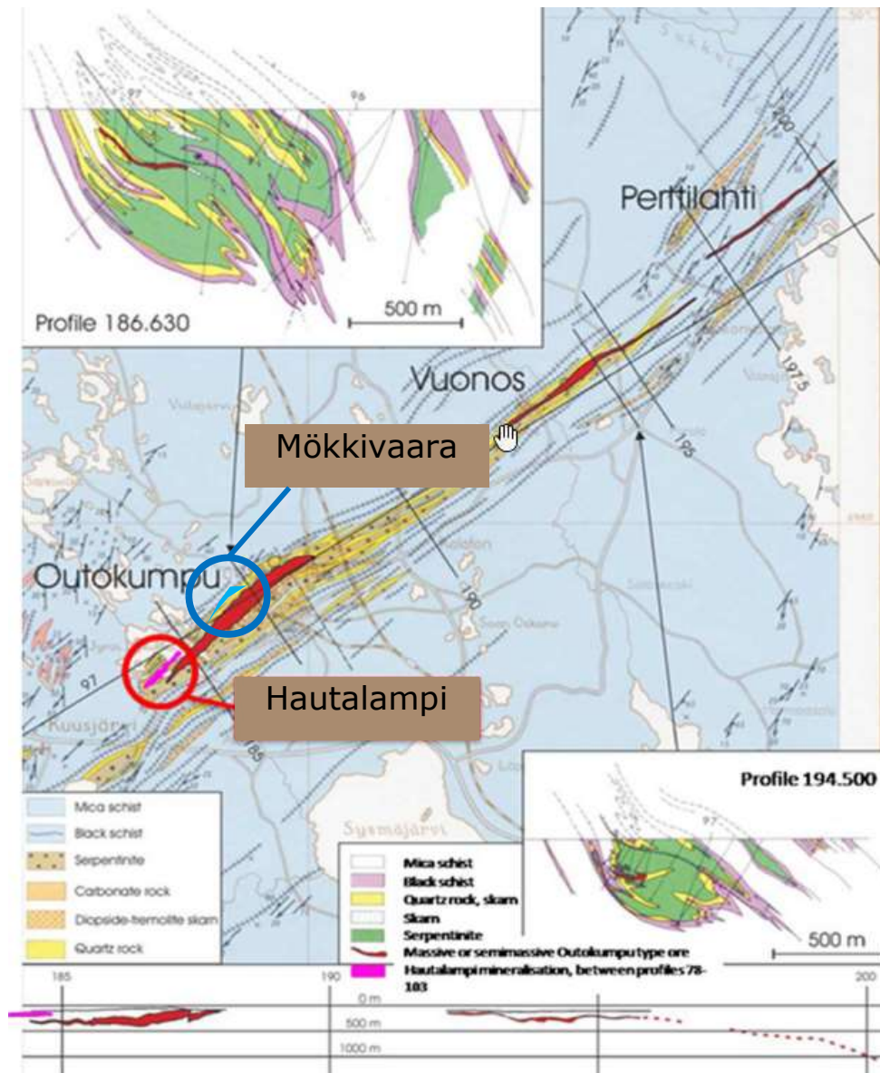
Figure 6-2 Geological map of the Outokumpu belt. Modified from GEOMEX report (2006) and Feasibility Study (2009)
