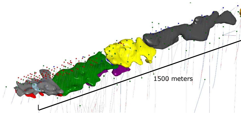
Figure 10-2 Oblique view of Hautalampi resource model. Looking towards North-East.
