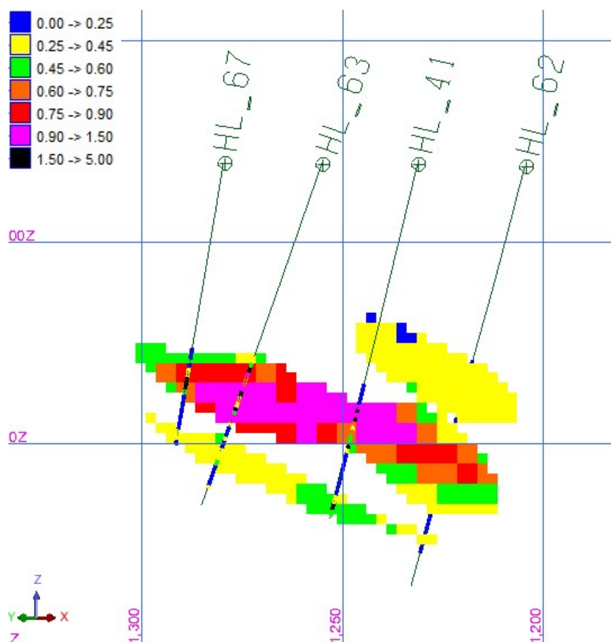
Figure 10-11 Profile 99+20m viewing North East displaying NiEq % grades in blocks and drill holes.
