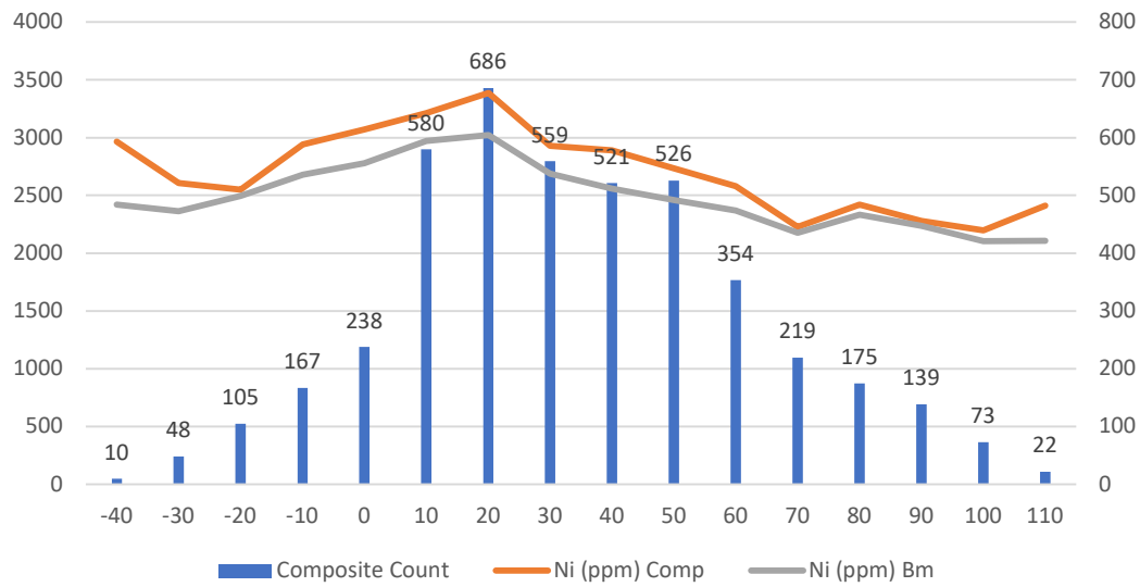
Figure 10-19 Swath Analysis: Ni, Elevation
