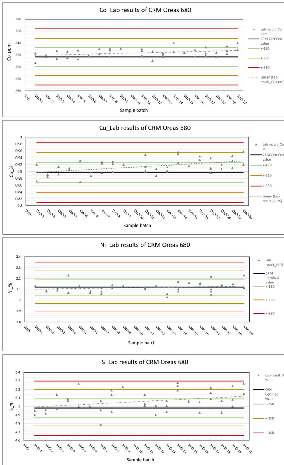
Figure 8-6 Assay results of standard Oreas 680, in chronological order.
