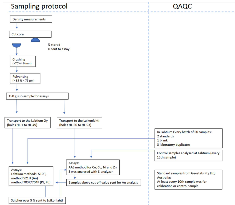
Figure 8-1 QAQC and Sampling protocol for Finn Nickel drill cores
