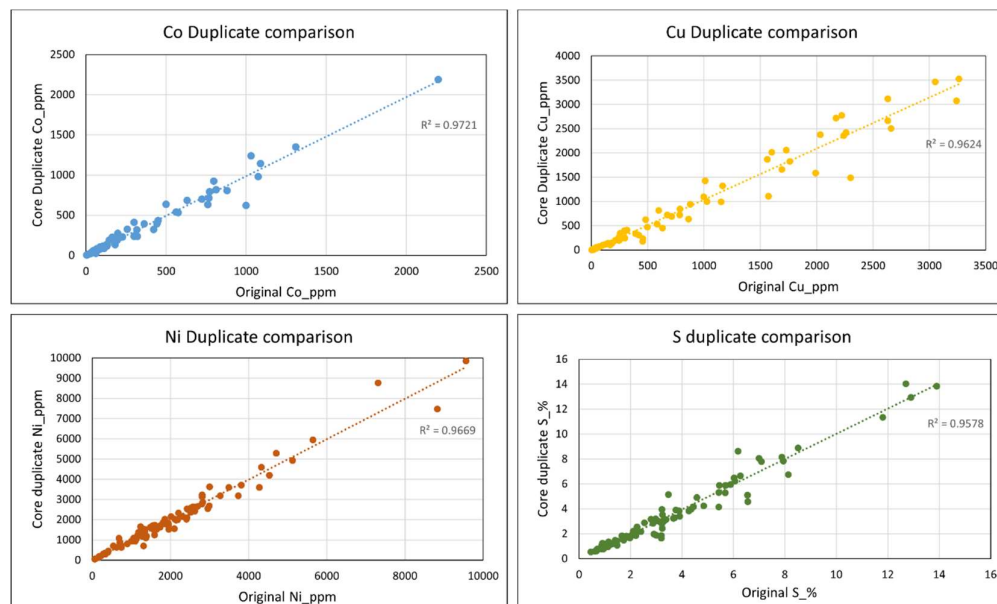
Figure 8-7 Assays of coarse duplicate samples plotted against their original counterparts.
