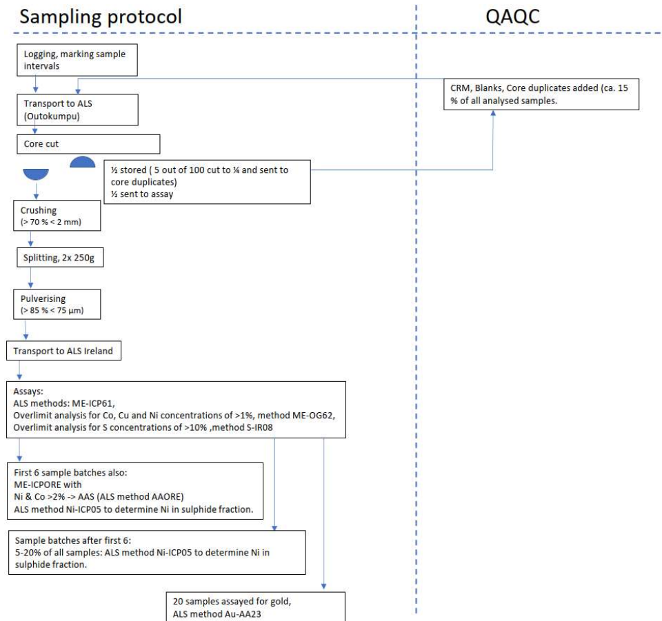
Figure 8-2 QAQC and Sampling protocol for FinnCobalt Oy's drill cores
