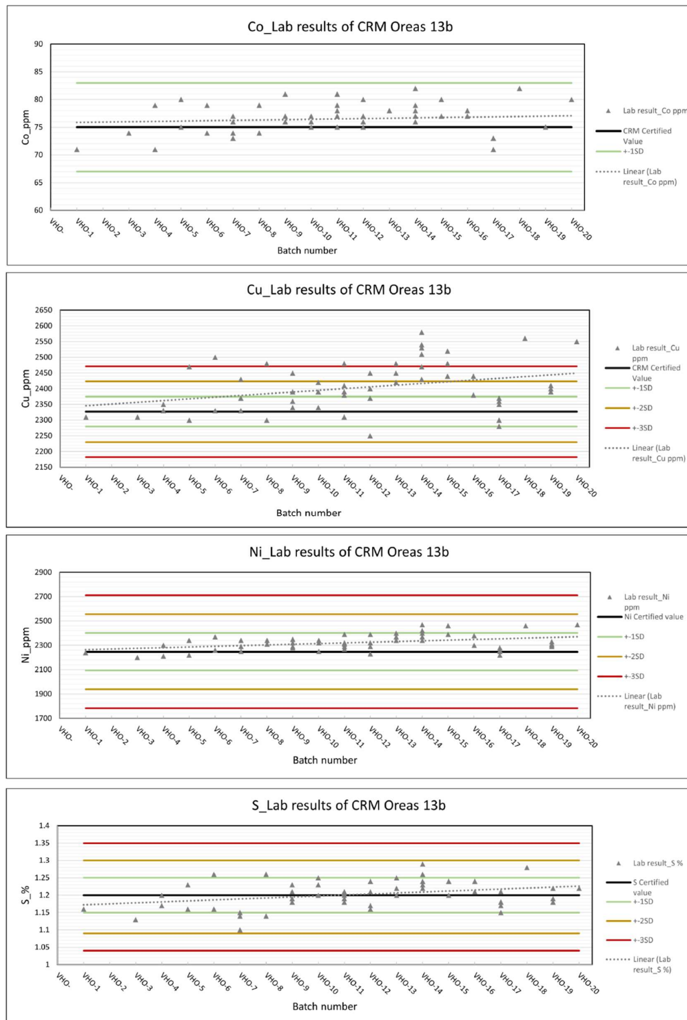
Figure 8-5 Assay results of standard Oreas 13b, in chronological order.
