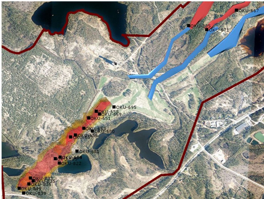
Figure 8-8 Location of the drill holes for the re-assays. Hautalampi resource area (red+yellow) and Blue-Sky areas / Mökkivaara (blue and red) are shown.
