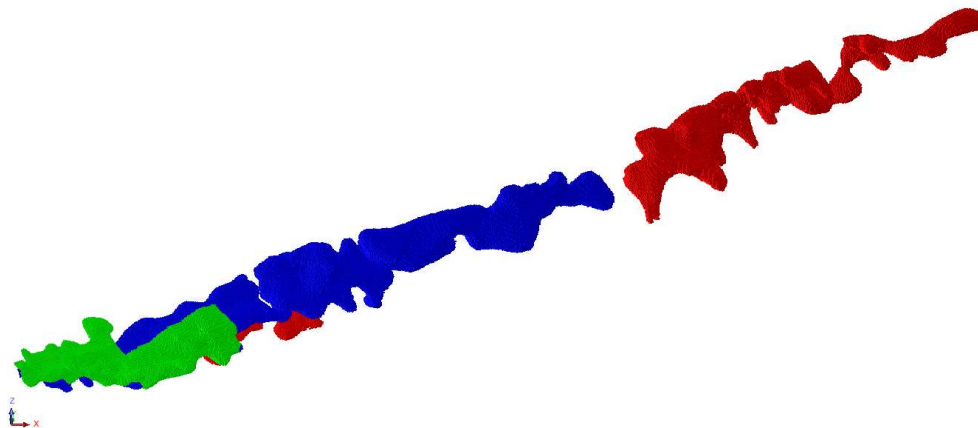
Figure 10-8 FinnCobalt Oy resources (Blue=Measured, Green= Indicated, Red =inferred resource class)
