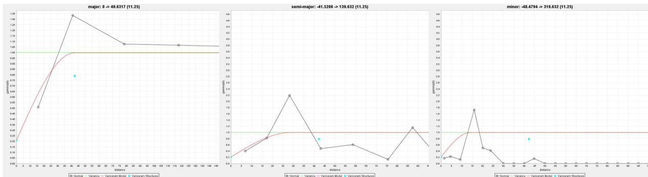
Figure 10-6 Experimental variogram models for Cu
