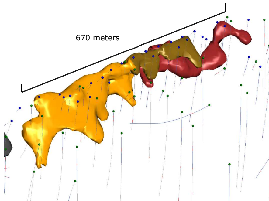
Figure 10-3 Oblique view of Mökkivaara resource model. Looking towards North-East.
