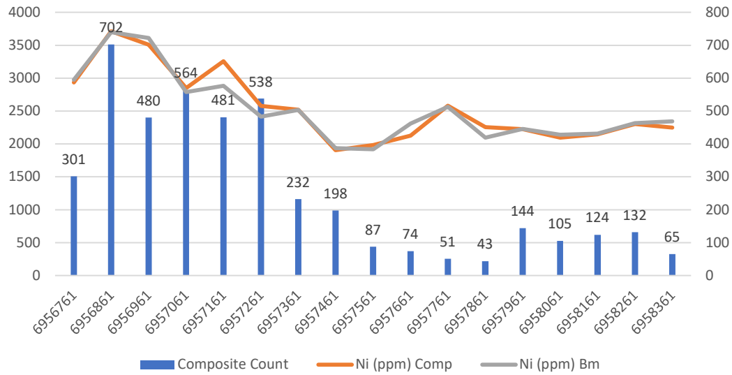
Figure 10-15 Swath Analysis: Co, Northing
