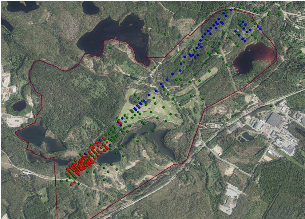
Figure 10-1 Drillholes from different drilling campaigns in relation to the mining concession. (Green=Outokumpu Oy, Red=Finn Nickel Oy, Blue = FinnCobalt Oy)
