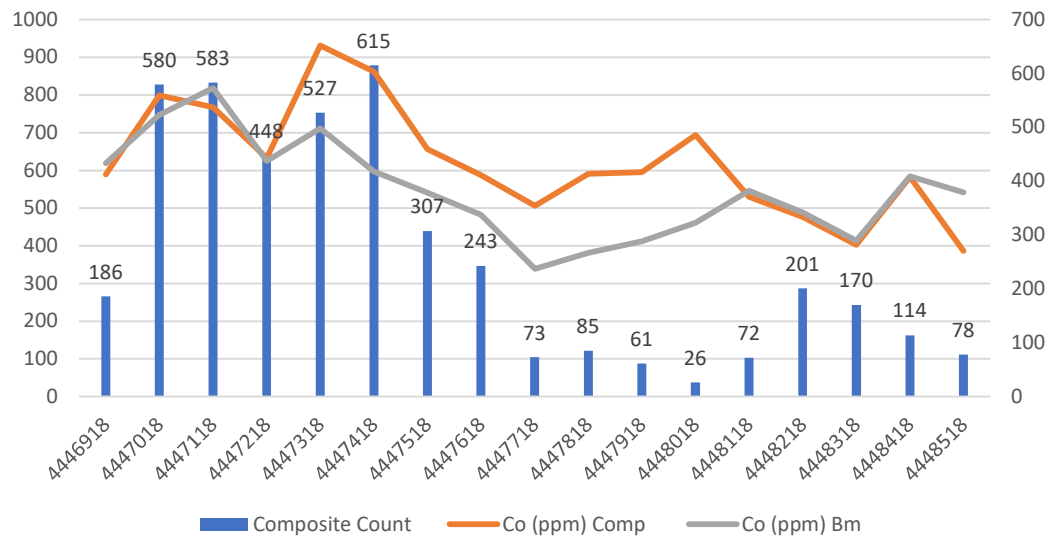
Figure 10-18 Swath Analysis: Co, Easting
