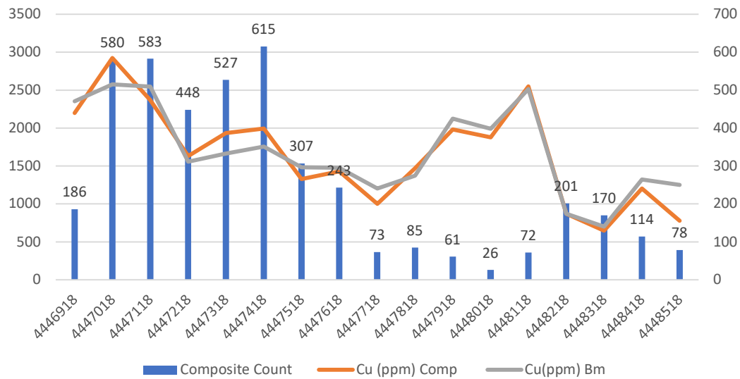
Figure 10-17 Swath Analysis: Cu, Easting
