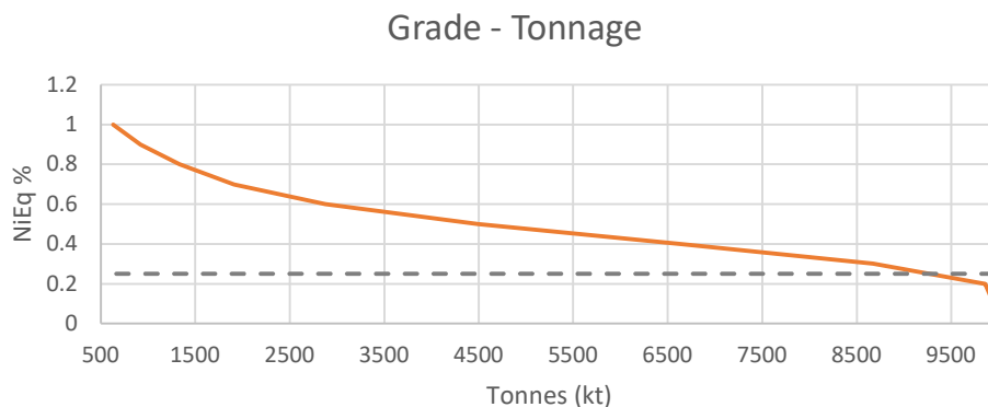
Figure 10-22 Hautalampi Grade-Tonnage curve for Measured & indicated resource class material, dashed line shows the selected cut-off.
