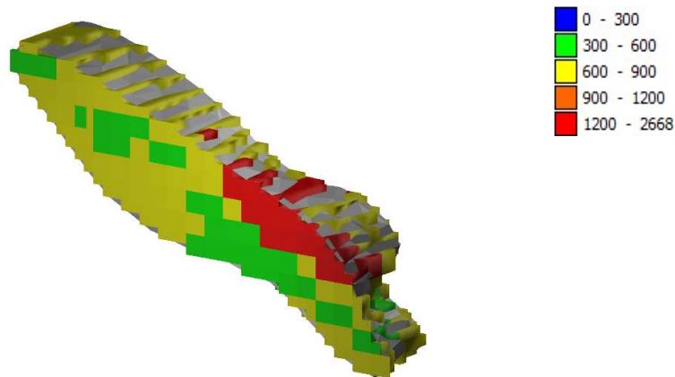
Figure 10-12 Volume comparison of 3D solid vs block model (Co grade)
