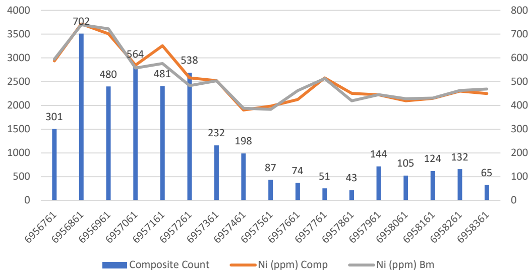
Figure 10-13 Swath Analysis: Ni, Northing
