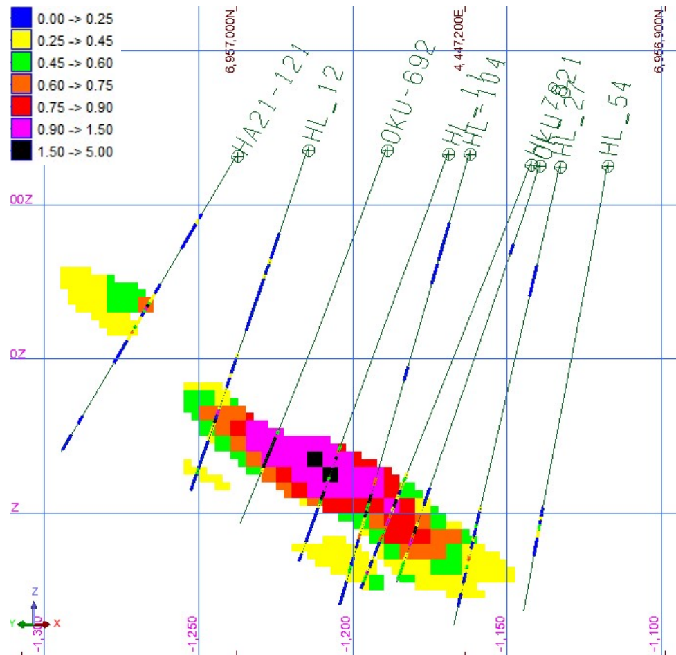
Figure 10-10 Profile 95 viewing North East displaying NiEq % in blocks and drill holes.
