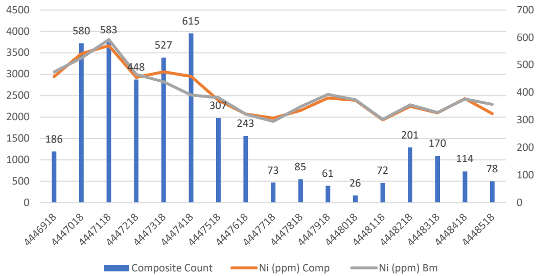
Figure 10-16 Swath Analysis: Ni, Easting
