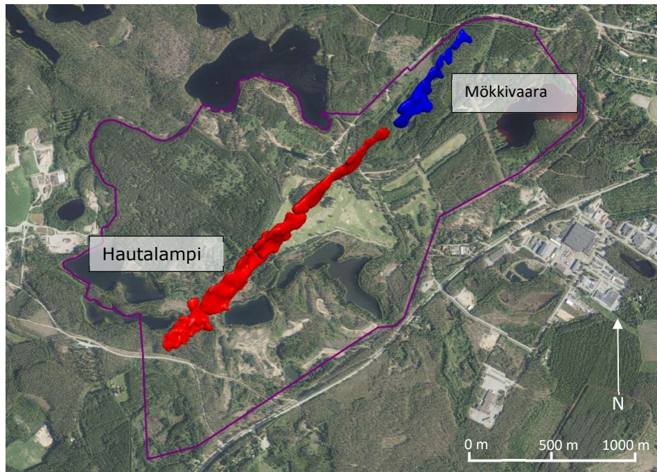
Figure 10-4 Aerial views of Hautalampi and Mökkivaara Resource models
